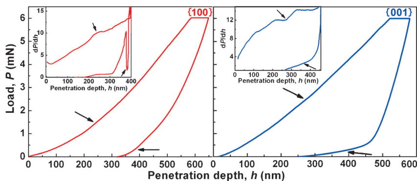
Figure 3. Representative P-h curves for 1 obtained from indentation with a spherical tip normal to the {100} and {001} facets. Inset: The derivative of the loading and unloading curves as a function of penetration depth for the weak “kink” and strong “elbow” events. The anomalies seen during loading and unloading are indicated with arrows.
